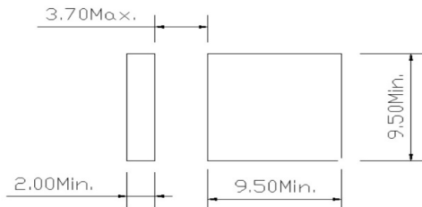
Recommended Foot Print in Millimeters
