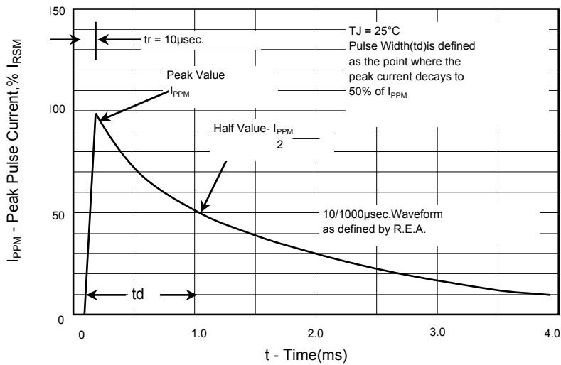
Fig.3 - Pulse Waveform
